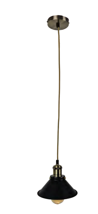
ITEM NO. B3610-180 805 THB Diameter W 18cm H 24cm Material Metal+Glass Input Voltage E27 220V Cable length 90 cm (Adjustable)
